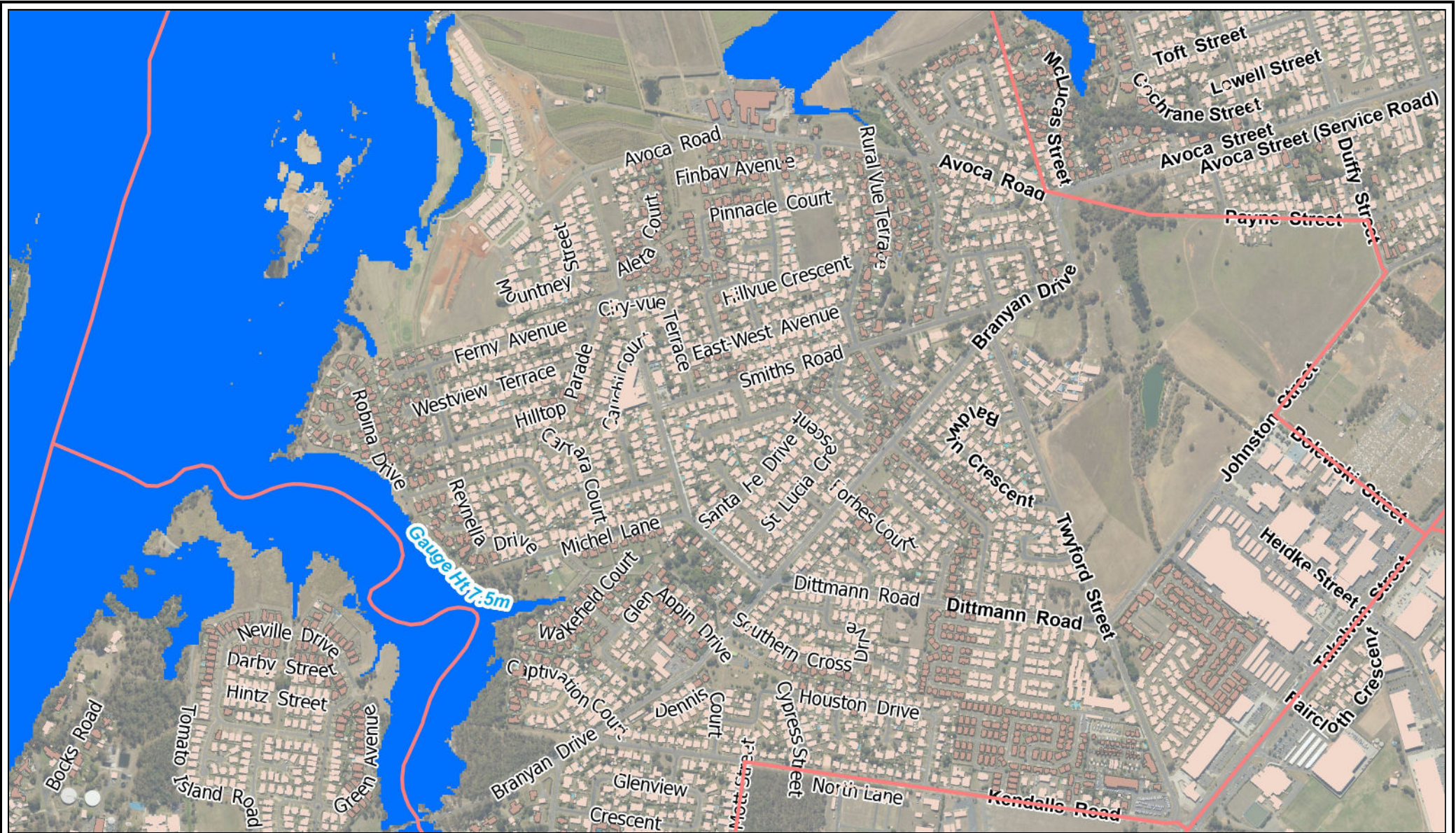
Predicted Peak Flood Extent - Bundaberg Gauge at 7.5m Avoca Focus
